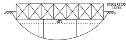
Fig 1.7: Semi-through Bridge
