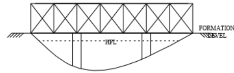
Fig 1.6: Through Bridge
