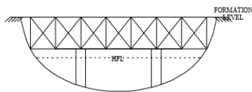
fig 1.5: Deck Bridge
